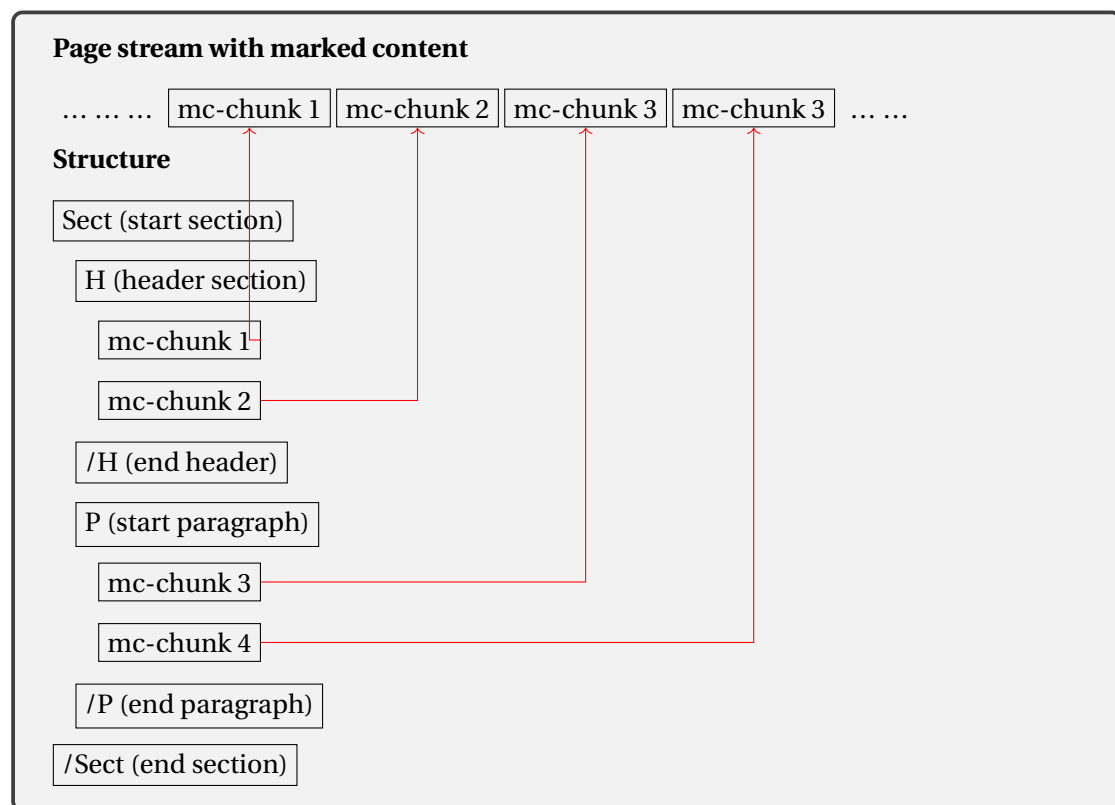
Figure 4: Schematic description of the relation between marked content in the page stream and the structure
